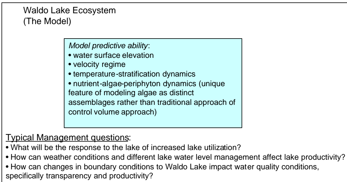
Figure 70: Model predictive ability coupled with water quality management issues.
