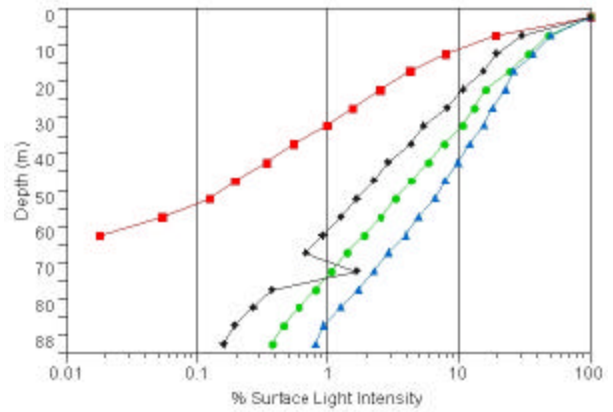
Figure 30: Attenuation of PAR, red, green, and blue wavelengths with depth in Waldo Lake in 2001 and 2002.
