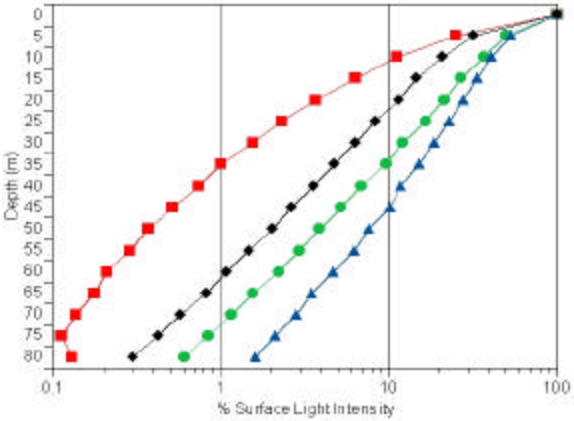
Figure 30: Attenuation of PAR, red, green, and blue wavelengths with depth in Waldo Lake in 2001 and 2002.
