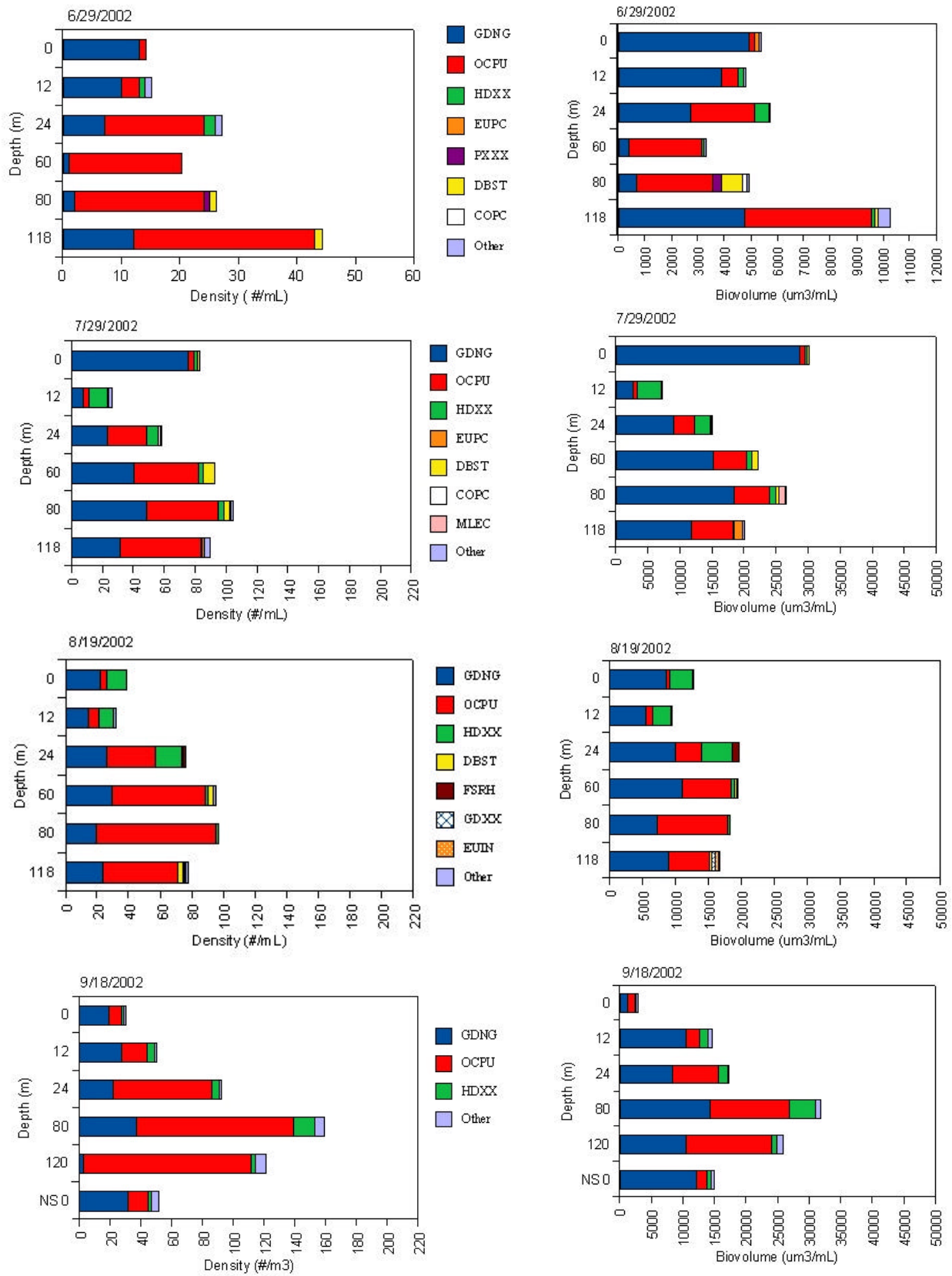
Figure 51: Vertical profiles of phytoplankton density (#/mL) and biovolume ( \mu\text{m}^3/\text{mL} ) in Waldo Lake in 2002 (species codes in Table 16). Note change in scale on 6/29/2002. “Other” indicates species representing less than 2 % of the total biovolume.
